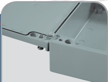
Integrated lid supports
