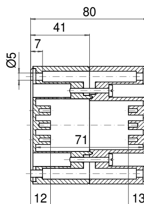
Maximum number of cable glands per enclosure side
